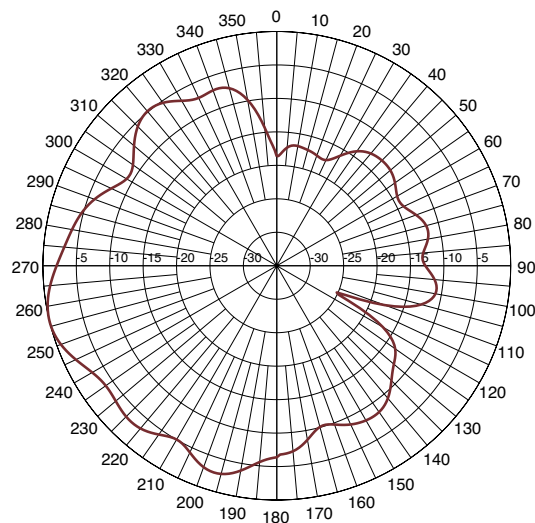
Azimuth Pattern at 5.2 GHz
