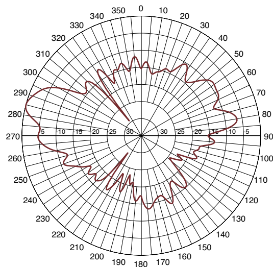
Elevation Pattern at 5.2 GHz
