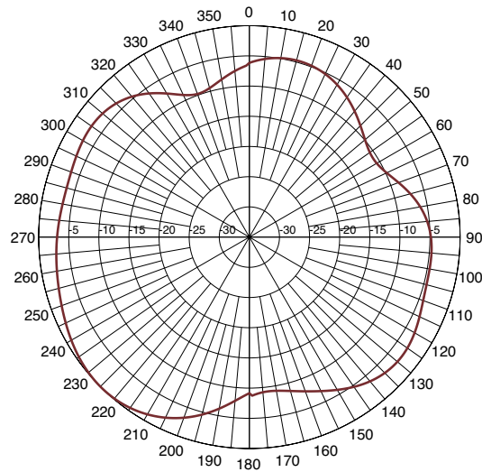
Azimuth Pattern at 2.45 GHz
