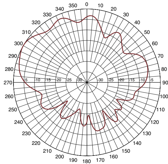
Elevation Pattern at 2.45 GHz
