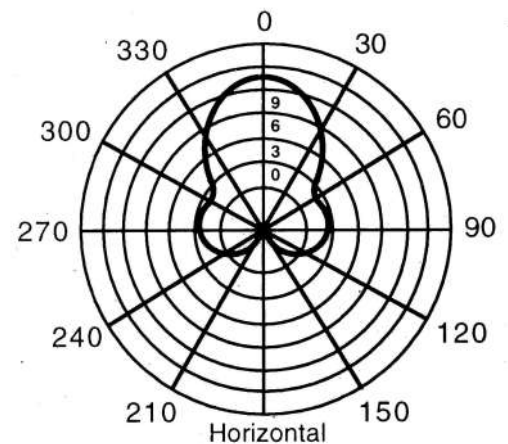
Radiation Patterns (Relative Field Strength) with Vertical Polarization
