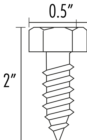
PIJA CABEZA HEXAGONAL 5/16" X 2"
