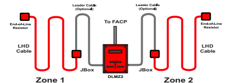
Typical System
