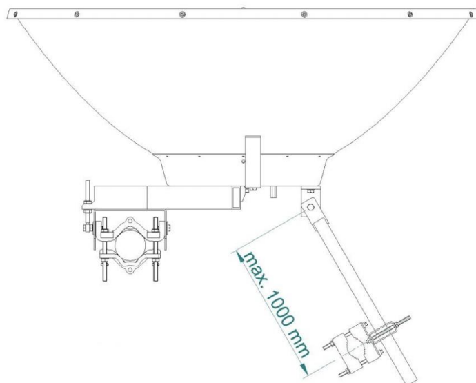
Fig. 3 Antenna with wind bracing set (top view)
