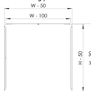
Mounting plate
